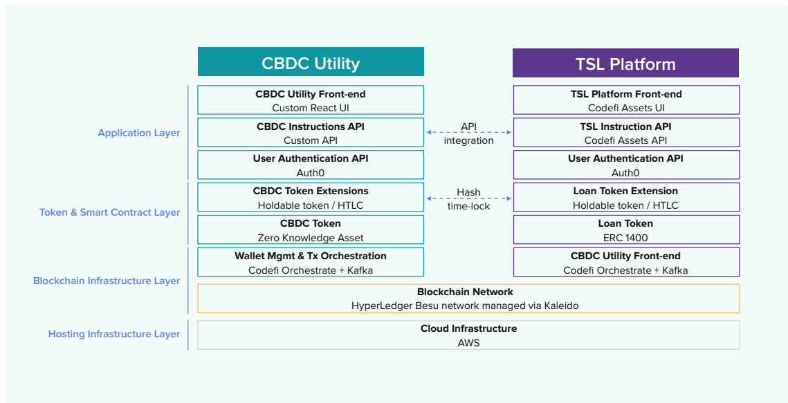
Figure 11: Technical Architecture
