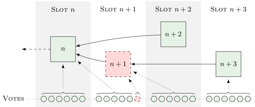
Fig. 1. Example of a one-block reorg attack using the refined strategy: In slot n+1 the adversary privately creates block n+1 on block n and attests to it. Honest validators of slot n+1 do not see any block and thus attest to block n as head of the chain. In the next slot, an honest proposer publishes block n+2 building on block n , which is the current head in their view. Simultaneously, the adversary finally publishes block n+1 and the attestation voting for block n+1 . All honest validators of slot n+2 attest to block n+1 as head of the chain, because it has more weight than block n+2 . In the next slot block n+3 is proposed building on block n+1 . Block n+2 is reorged out.
