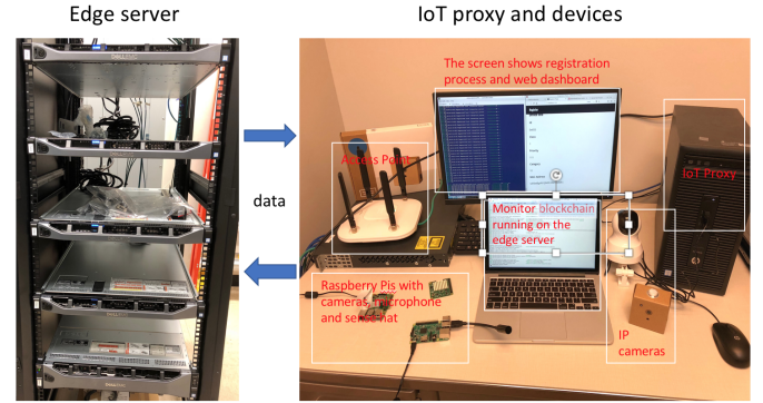
Fig. 9: EdgeChain testbed.
