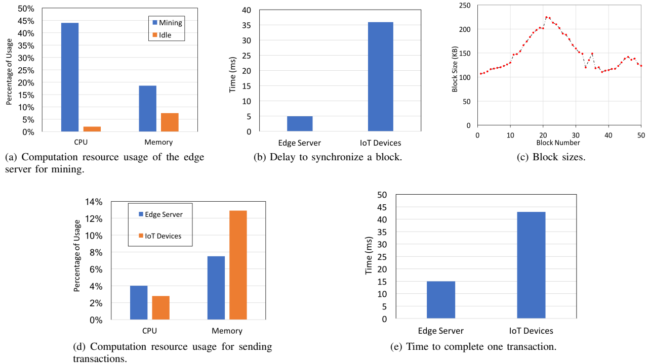
Fig. 11: Overhead of system operation.
