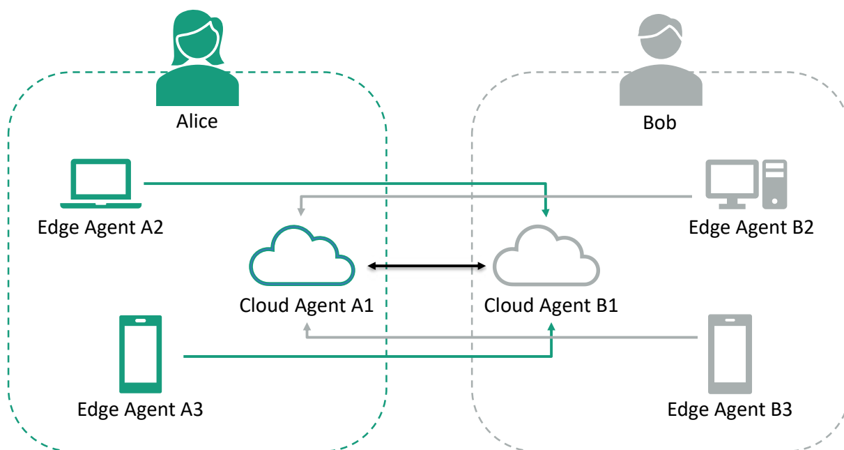
Figure 9: Agent-to-Agent communication
