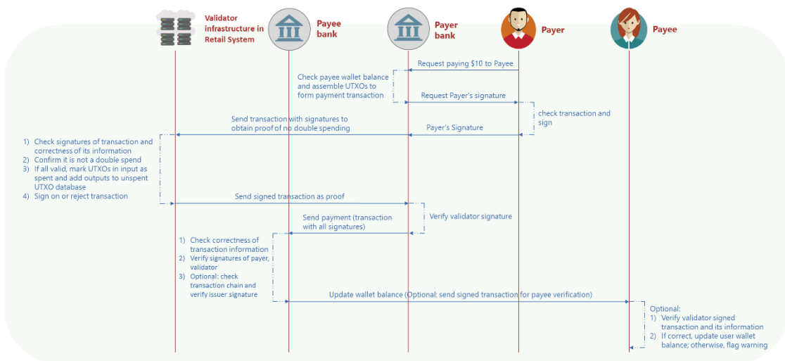
Figure 10. Transaction flow for retail payment transaction between users
