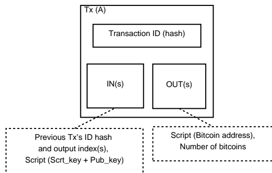
Fig. 2. Bitcoin transactions
