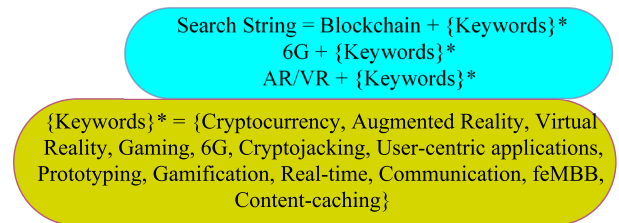
FIGURE 4. Search Strings.
