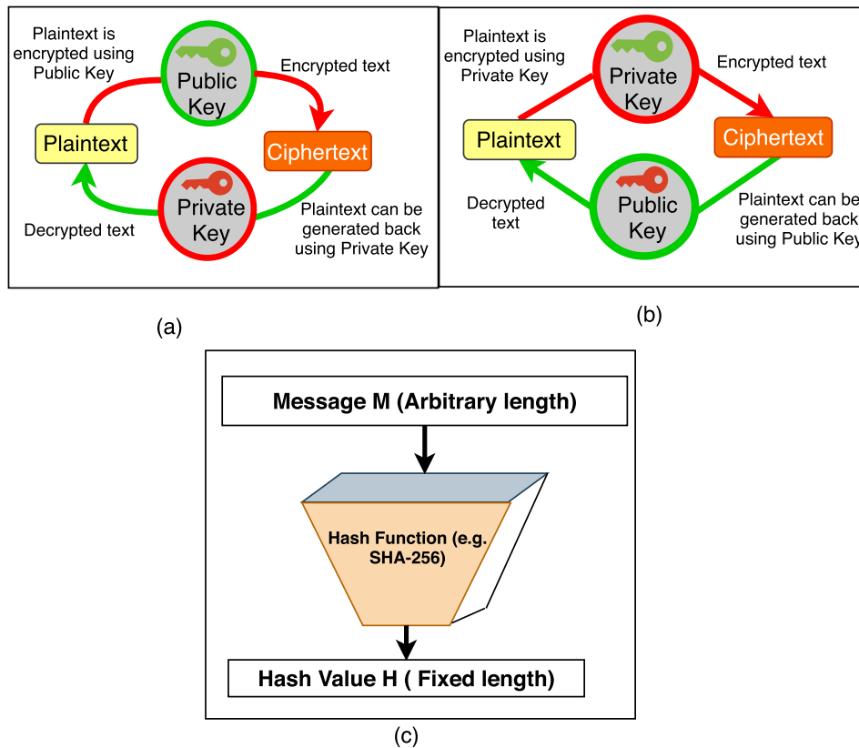
Fig. 6. The properties of public and private key pairs. (a) demonstrates that a message is encrypted with a public key, a private key is utilized to decrypt the message. (b) shows that the ciphertext of the message is generated using private key and plaintext is produced using the public key. (c) depicts a cryptographic hash function which is a mathematical algorithm that takes an arbitrary amount of data input to map the content to a bit array of a fixed size called hash value or just a “hash”.
