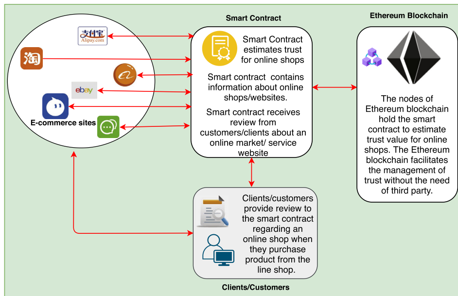
Fig. 10. Example of a smart contract application.
