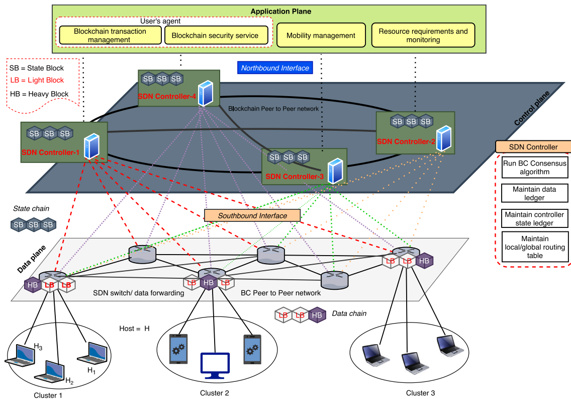
Fig. 17. The blockchain enabled decentralized SDN (Software-Defined Networks) architecture for IoT (Internet of Things).
