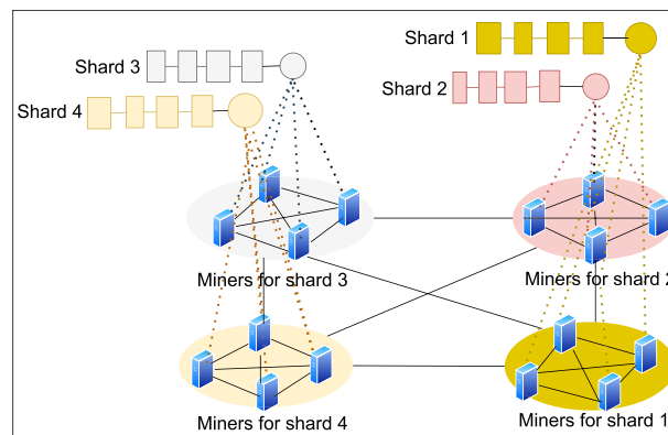
Fig. 9. Example of a blockchain sharding.
