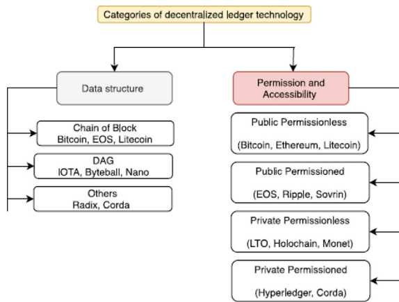
Fig. 11. The types of decentralized ledger technology. DAG: distributed acyclic graph.
