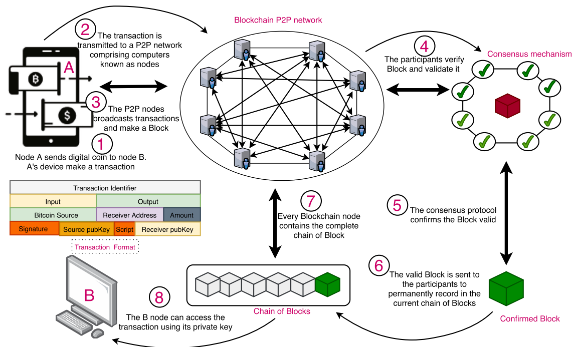
Fig. 2. The basic operation of Bitcoin blockchain (adopted from Ref. [35] with permission). P2P: peer to peer. Here, the superscript in front of the bullet points is mapped to the different steps of Fig. 2.
