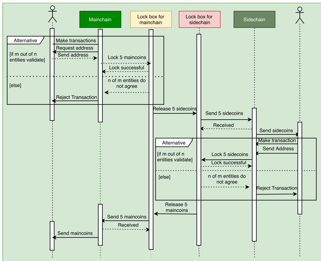
Fig. 13. The sequence diagram of two-way peg communication.
