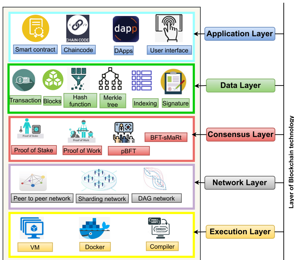
Fig. 3. The layered structure of blockchain technology. pBFT: Practical Byzantine Fault Tolerance; DAG: Distributed Acyclic Graph; VM: Virtual Machine.
