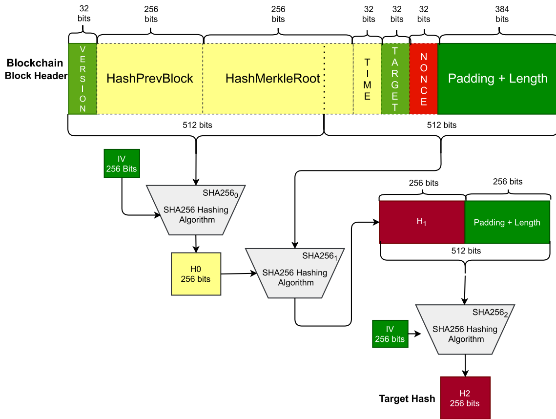
Fig. 5. The bitcoin block header hashing algorithm (adopted from Ref. [40] with permission).
