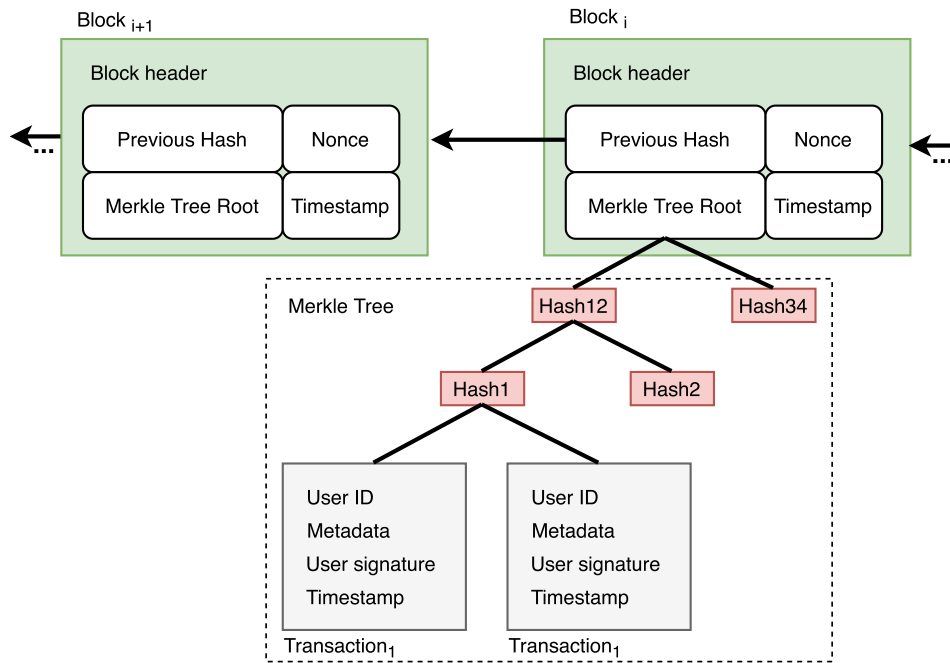
Fig. 4. The structure of a block.
