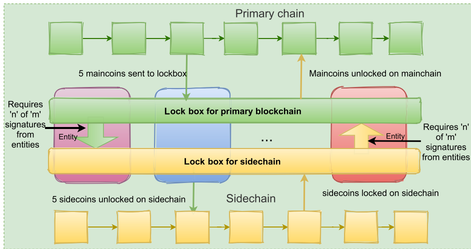
Fig. 12. The Federated two-way peg communication.
