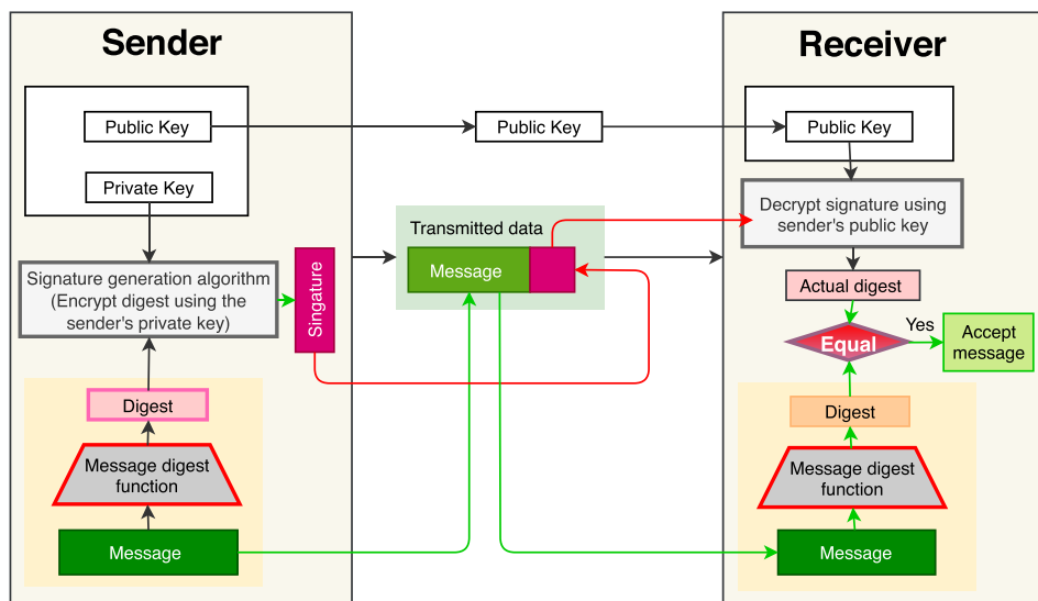
Fig. 7. The processing of forming and verifying digital signature in Bitcoin blockchain.
