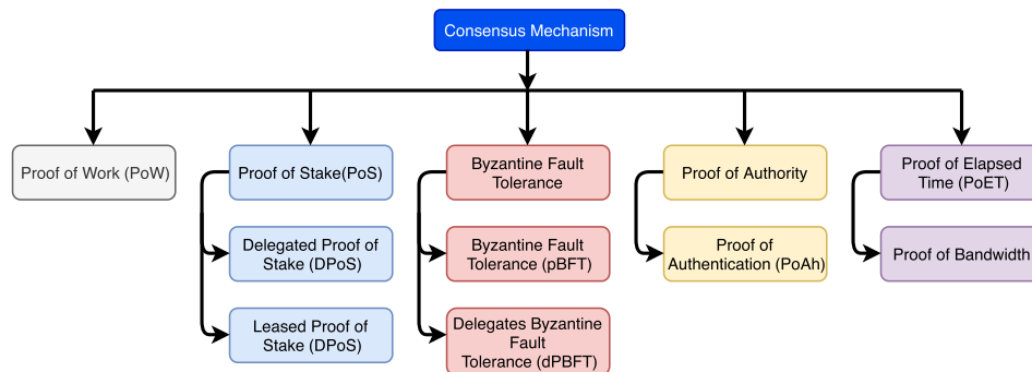
Fig. 8. The taxonomy of consensus mechanism.
