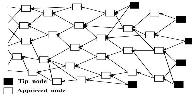
Fig. 3: Tangle protocol
