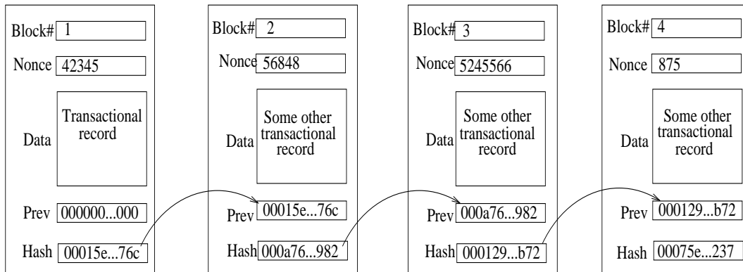
Fig. 1: Chaining of blocks in blockchain
