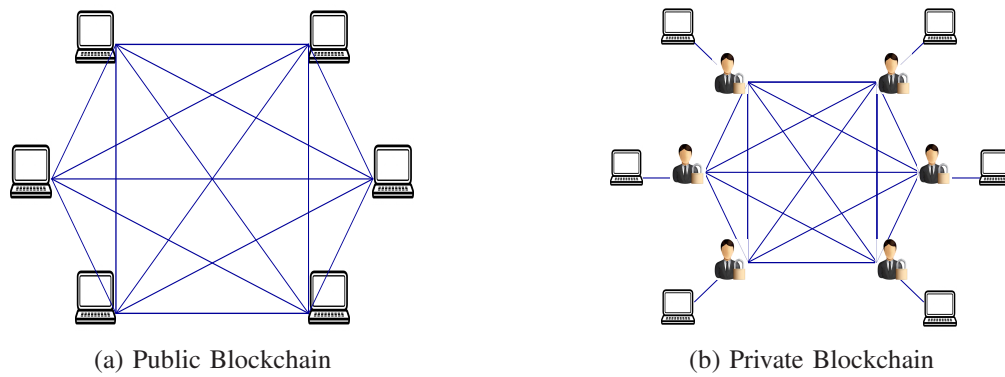
Fig. 2: Public blockchain vs private blockchain. In private blockchain, users' access to the blockchain is restricted by an institution.
