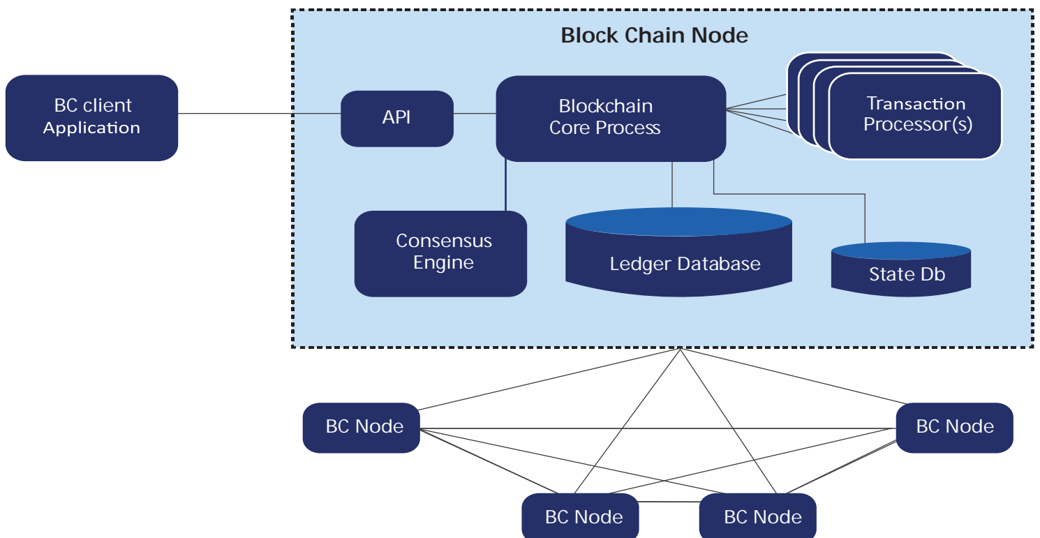
Figure 1 – Blockchain ecosystem
