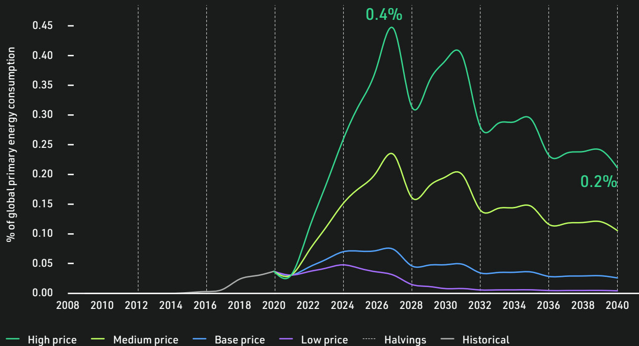
Historical and projected 1 Bitcoin electricity consumption as a percentage of global primary energy consumption %, 2009 - 2040
