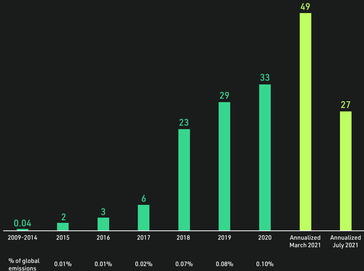
CHART 14: Carbon emissions from electricity consumed in Bitcoin mining MtCO 2 , 2009 – 2021
