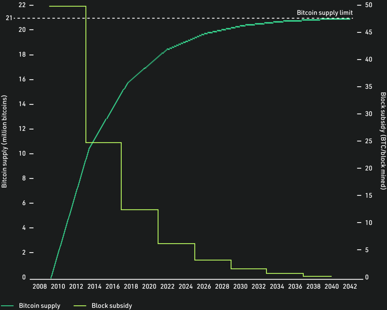
CHART 17: Total mined Bitcoin supply and block subsidy by year Million bitcoins, BTC/block subsidy, 2009 – 2040
