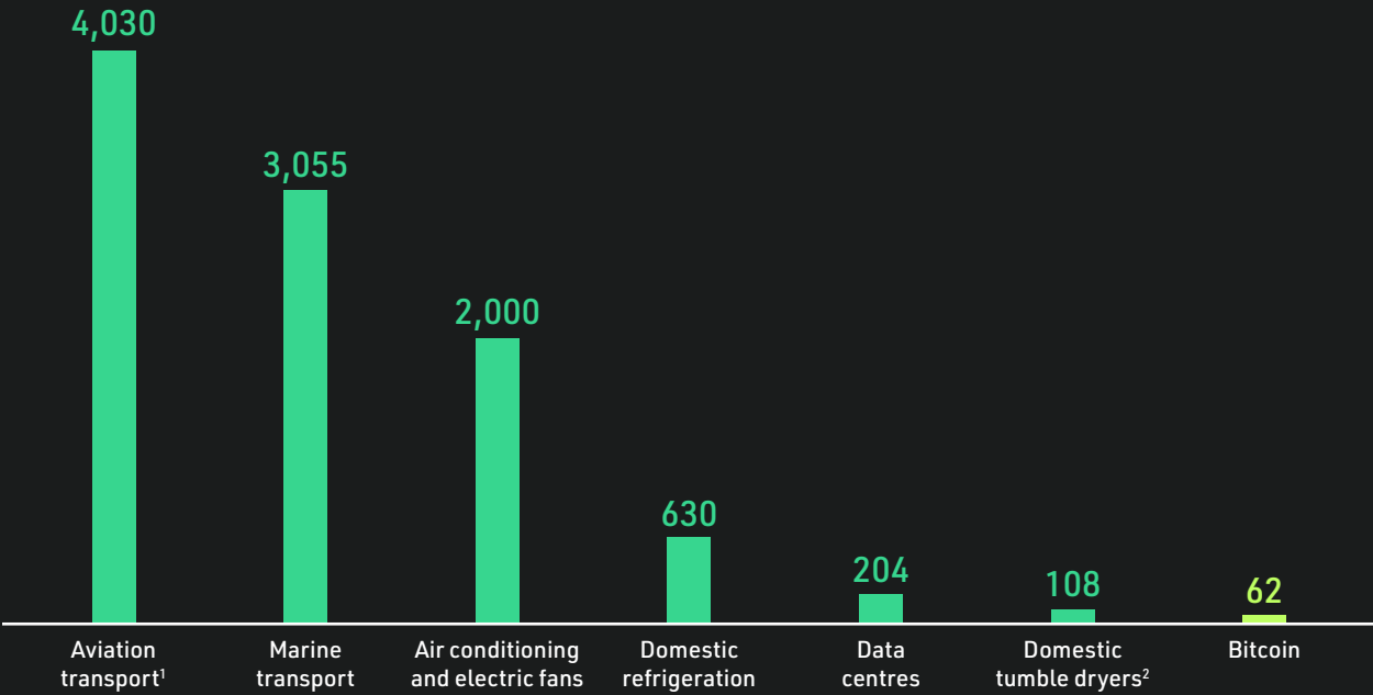
CHART 15: Energy consumption of Bitcoin mining versus other innovations TWh, 2020
