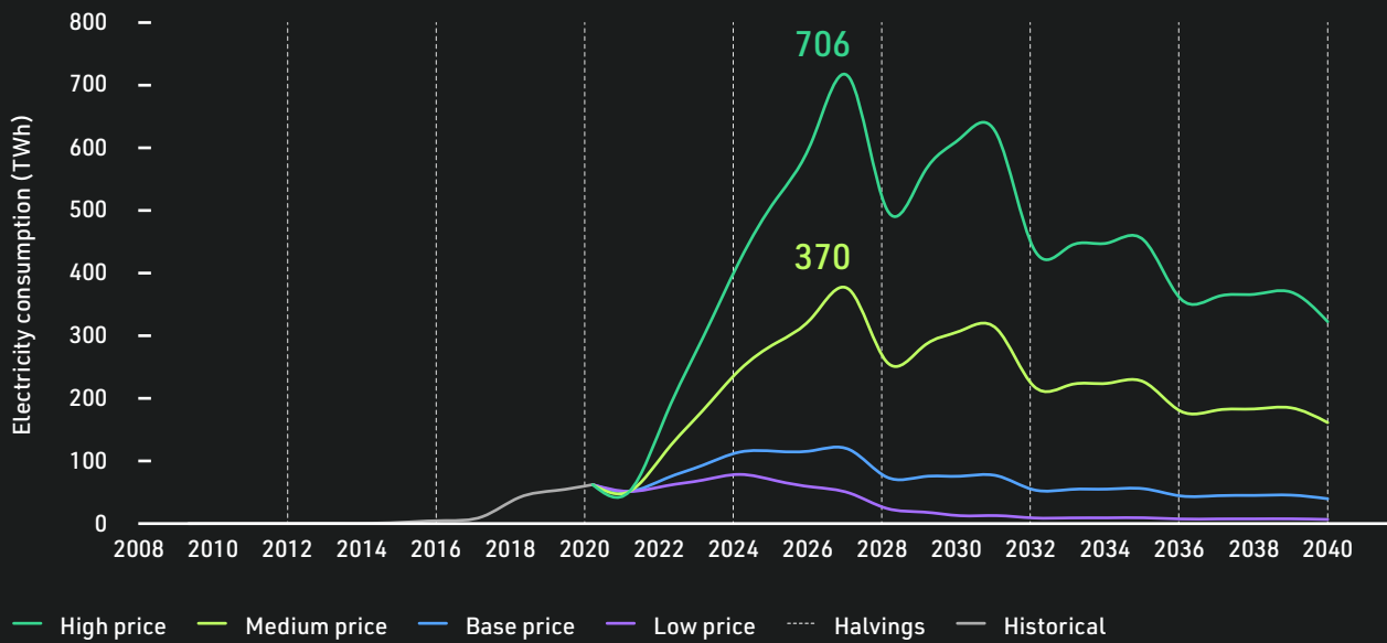
Historical and projected 1 Bitcoin electricity consumption under four price scenarios TWh, %, 2009 - 2040
