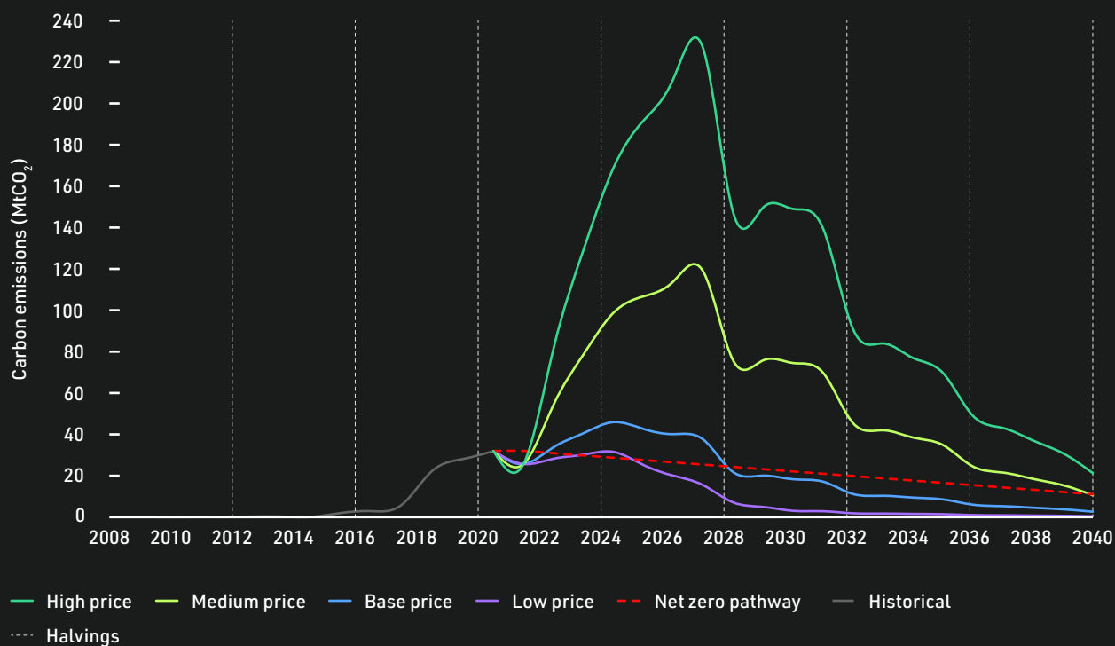
CHART 25: Historical and projected 1 Bitcoin carbon emissions under four price scenarios compared to net zero pathway 2 MtCO 2 , %, 2009 – 2040
