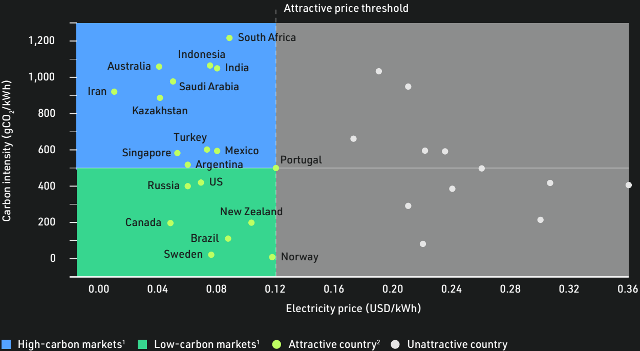
CHART 22: Average electricity price and carbon intensity for selected regions gCO 2 /kWh, USD/kWh, 2020
