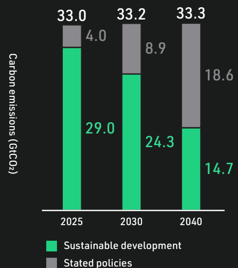
Projected Carbon Emissions: IEA 2020 Sustainability scenario GtCO 2
