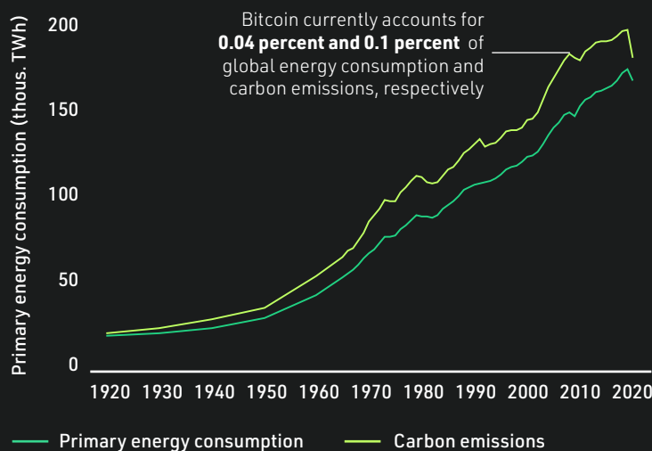
Historical 1 global primary energy consumption and carbon emissions Thous. TWh, GtCO 2 , 1920-2020
